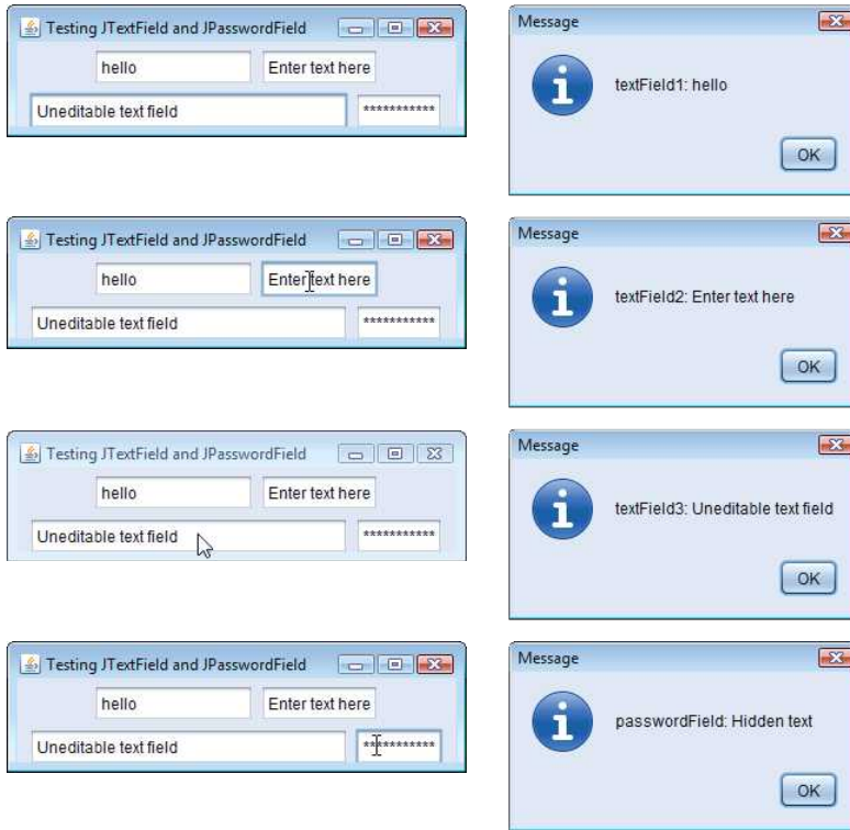
Fig. 12.10 | Testing JTextFieldFrame. (Part 2 of 2.)
