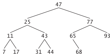
Fig. 21.16 | Binary search tree containing 12 values.
