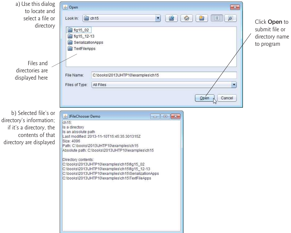
Fig. 15.13 | Testing class FileDemonstration . (Part 2 of 2.)
