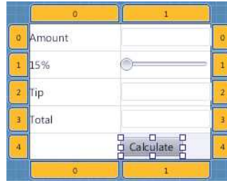
Fig. 25.13 | GridPane filled with the Tip Calculator’s controls.
